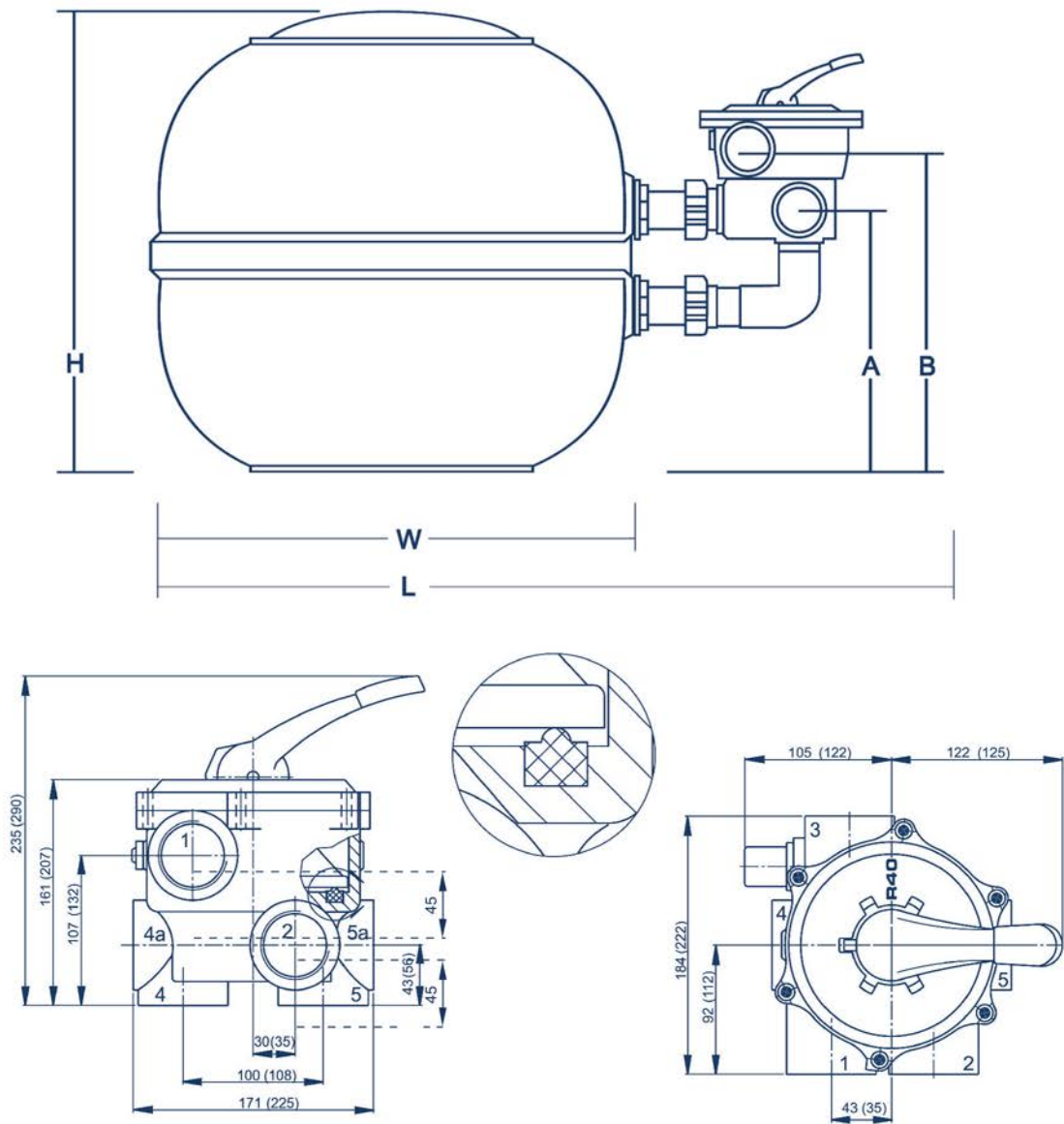
AQUASWIM® range dimension table (mm) / AQUASWIM®-afmetingstabel (mm)
